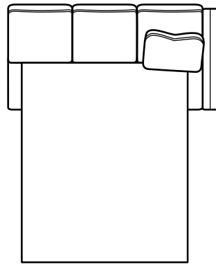
550-017 RSF Queen Sleeper* 77 W 38 D 35 H 29 AH 21 SH
